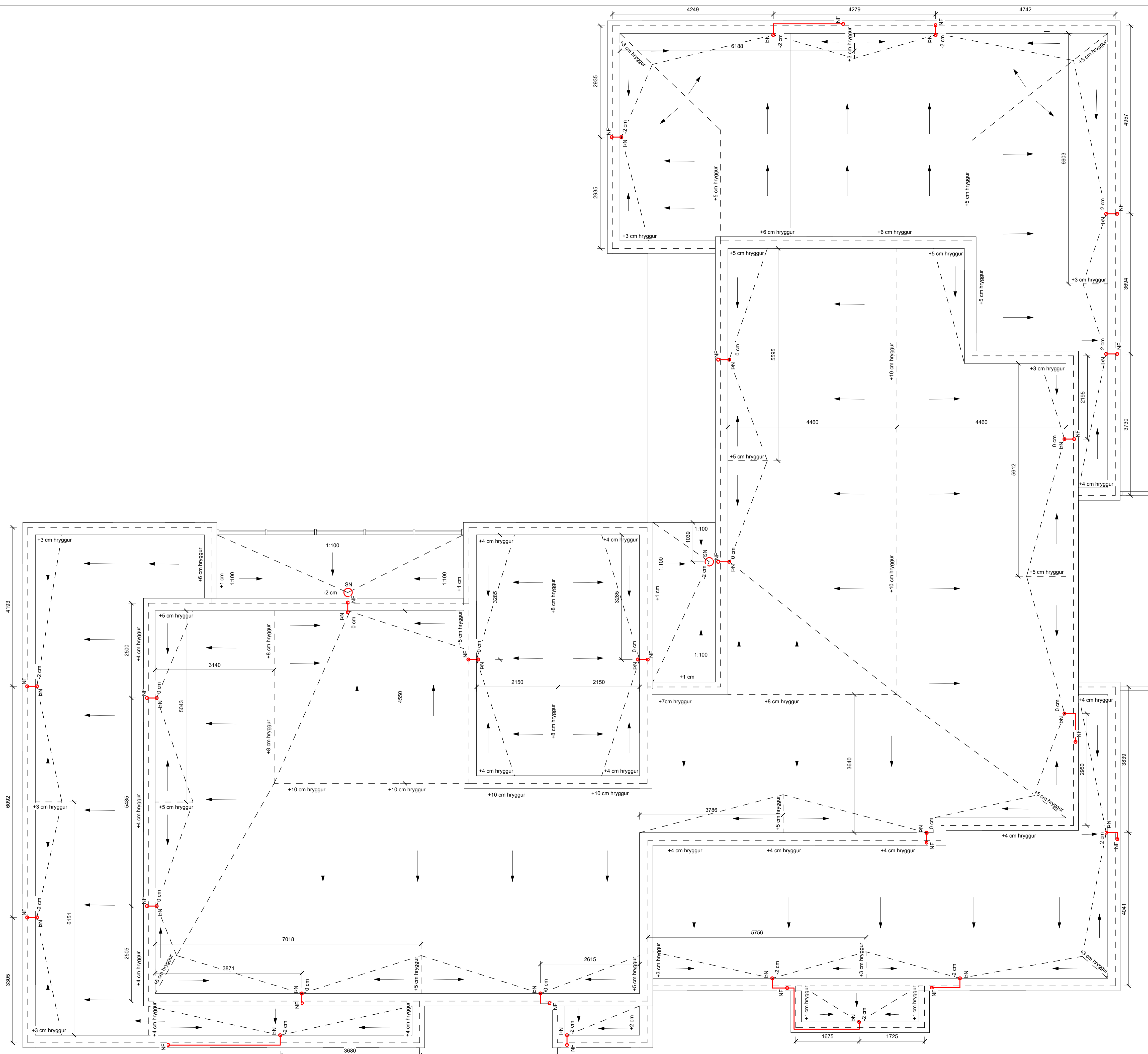
ÞAKHALLAPLAN mkv: 1 : 50
